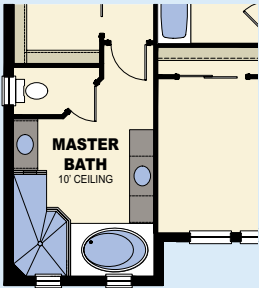
OPTIONAL ALTERNATE MASTER BATH W/ GARDEN TUB
